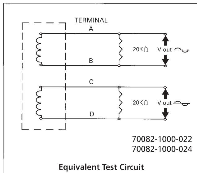
Dual Coil
